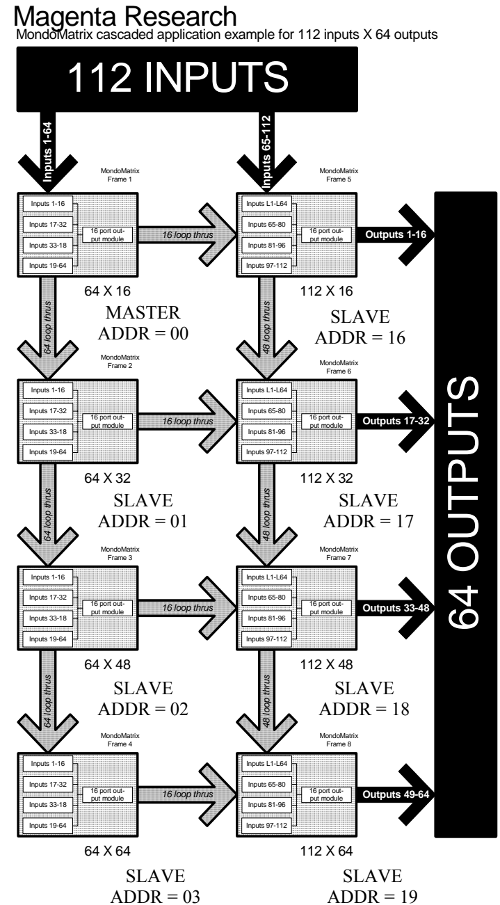
Figure 2-1 Mondo Matrix Sample Application for a 112 by 64 matrix
